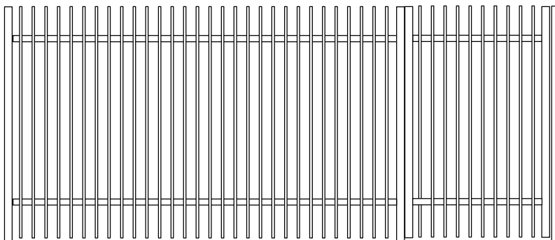
Blade (Aluminium 65x16mm) @ 81mm centres
