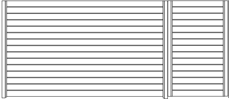
Visage Slat / 90mm @ 100mm centres
